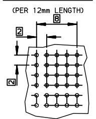
LAYOUT FOR P.C.B
